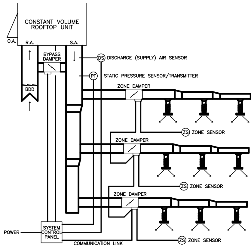
Figure 12.1 Constant volume rooftop unit serving an RTU zoning system.
