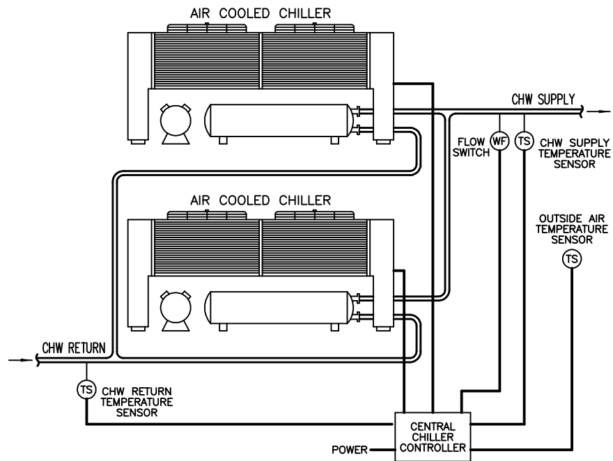
Figure 18.5 Two air cooled chillers serving a common chilled water system, controlled by an outboard central chiller controller.
