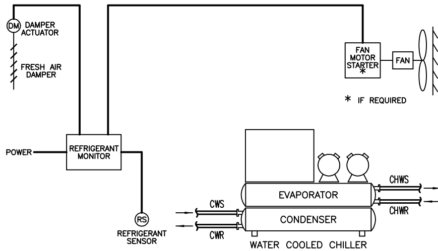
Figure 18.6 Refrigerant monitoring system consisting of a refrigerant monitor/sensor, an exhaust fan, and a motorized fresh air intake damper.
