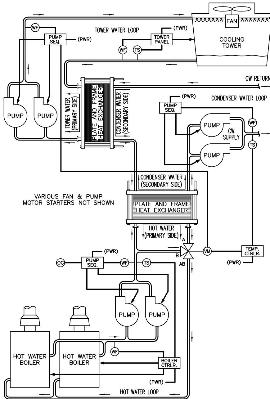
Figure 23.3 "Three loop" system.
