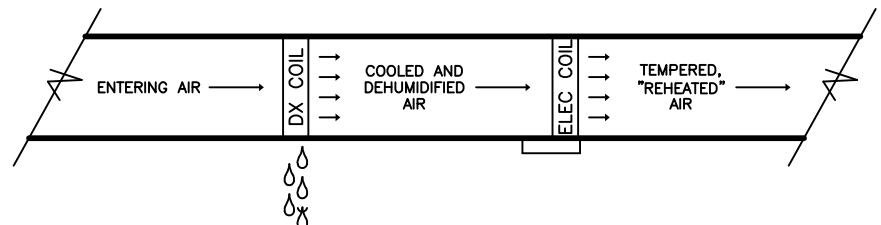
Figure 6.5 Direct expansion and electric heating coils employed in a dehumidification cycle.
