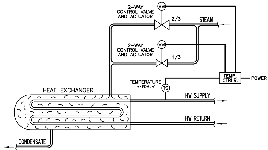
Figure 6.3 1/3, 2/3 control of a steam-to-hot water heat exchanger, performed by an electronic temperature controller.
