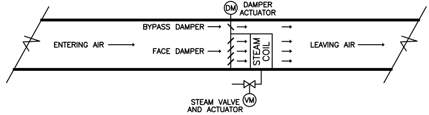
Figure 6.4 Steam coil equipped with a face/bypass damper assembly.
